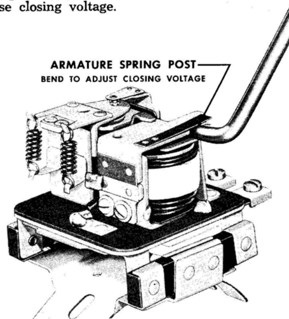
Figure 11—Adjustment of cutout relay closing voltage (1118200 series).
