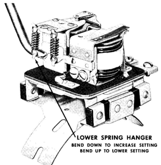
Figure 15—Adjusting voltage setting of current-voltage regulator unit (1118200 series).
