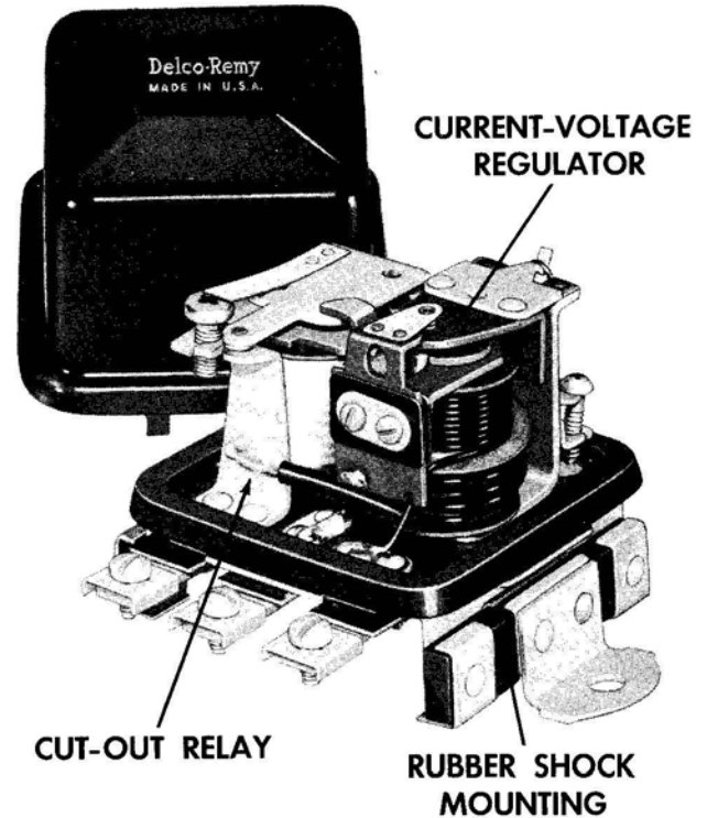
Figure 2—Delco-Remy 1118300 and 1118700 type combined current-voltage regulator with cover removed so units can be seen.
