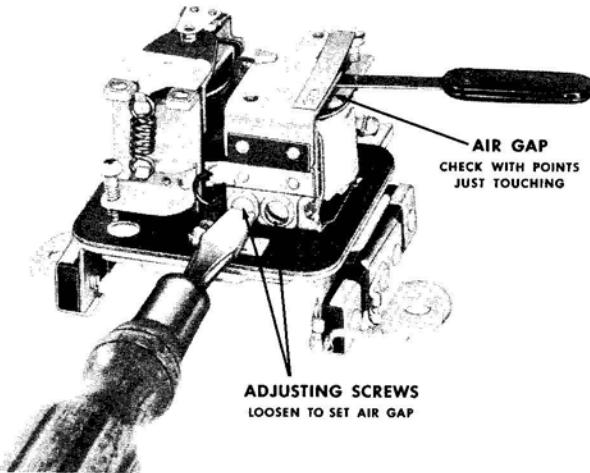
Figure 8—Cutout relay air gap check and adjustment (1118300 and 1118700 series). Battery must be disconnected when this check is made.
