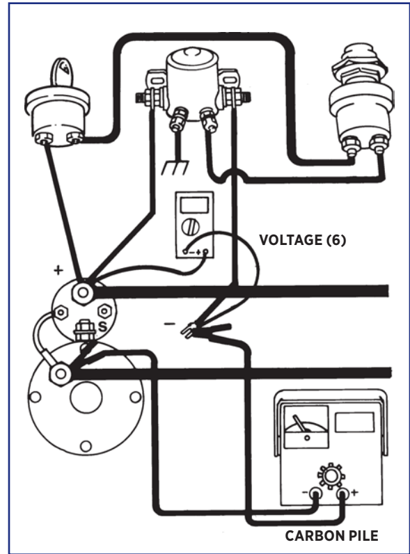
FIGURE 3-5. Starter Solenoid Circuit Test
